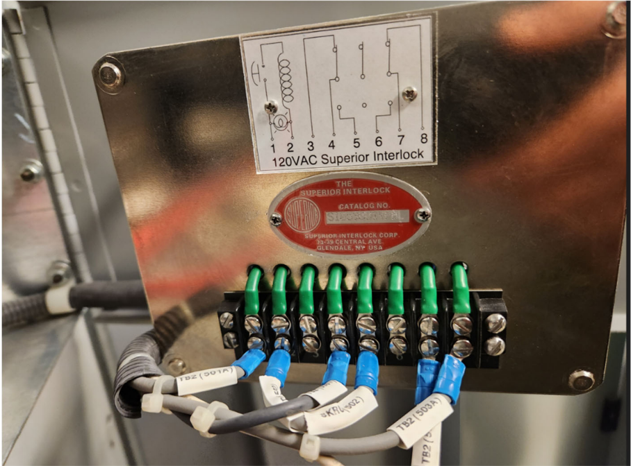
Figure 10: SKRU (Solenoid Key Release Unit)
