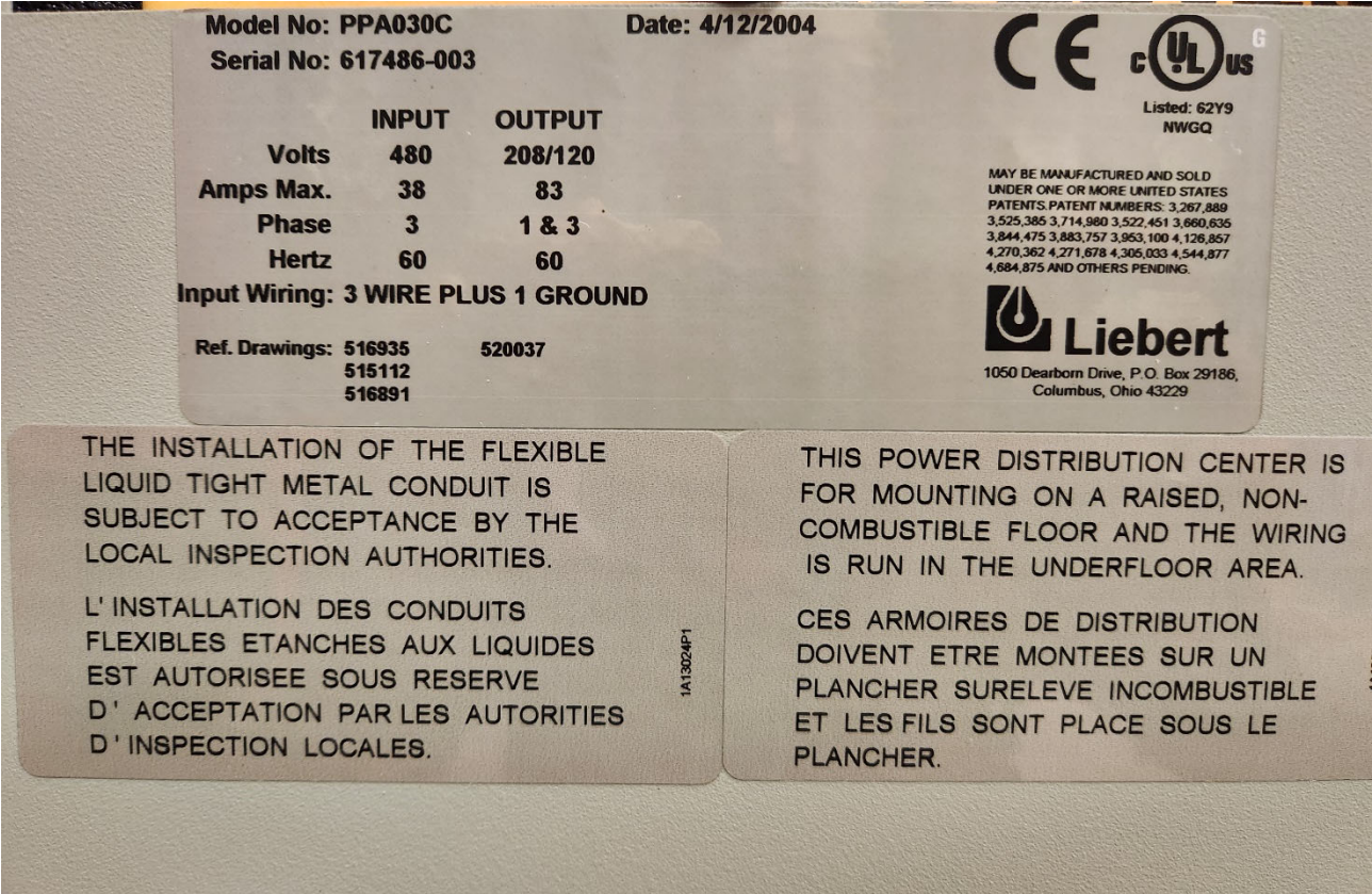
Figure 12: PDA Nameplate
